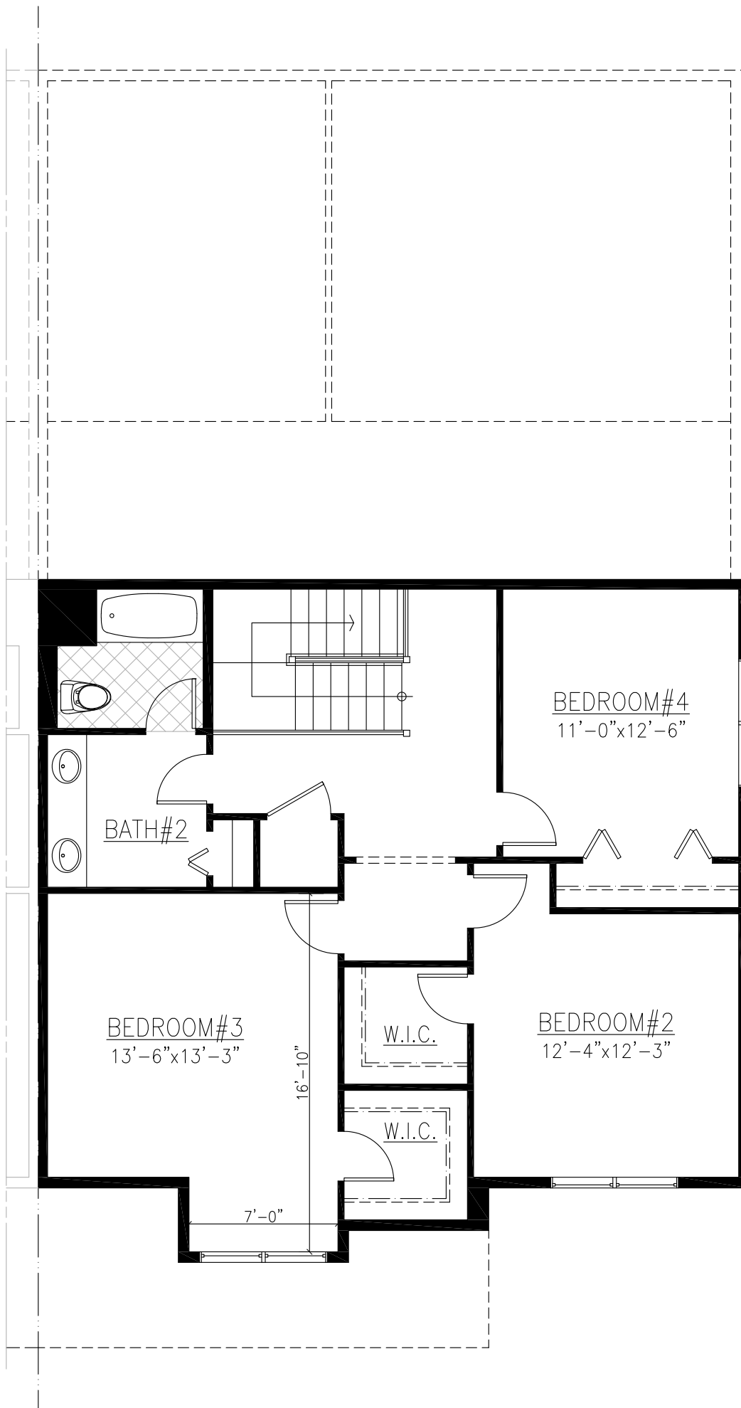
Second Floor Plan Drawing
