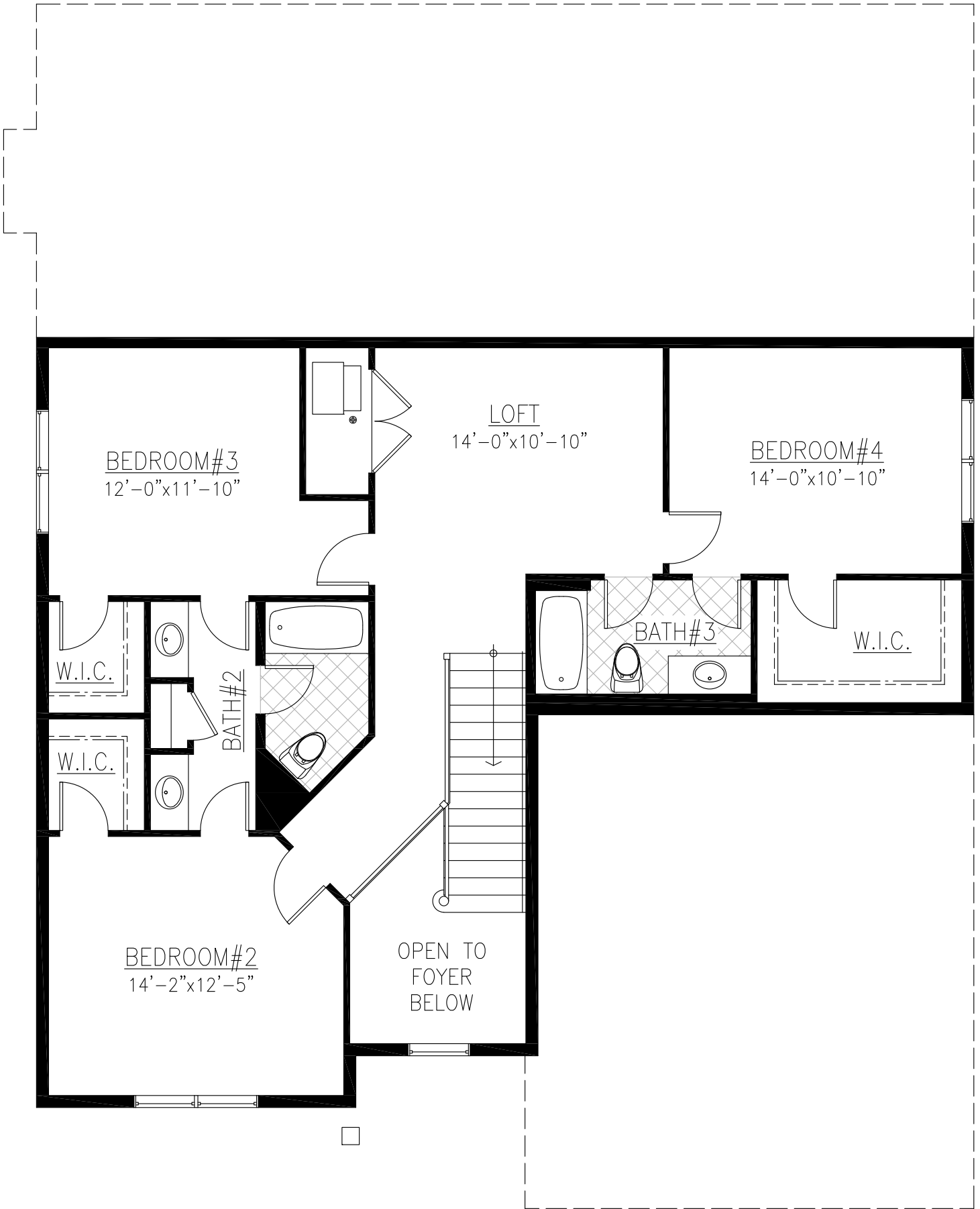
Second Floor Plan Drawing
