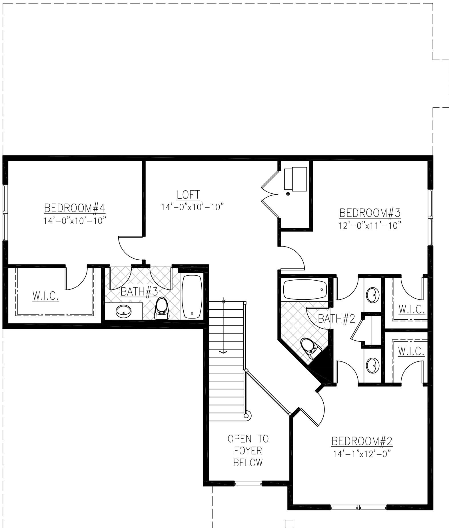
Second Floor Plan Drawing
