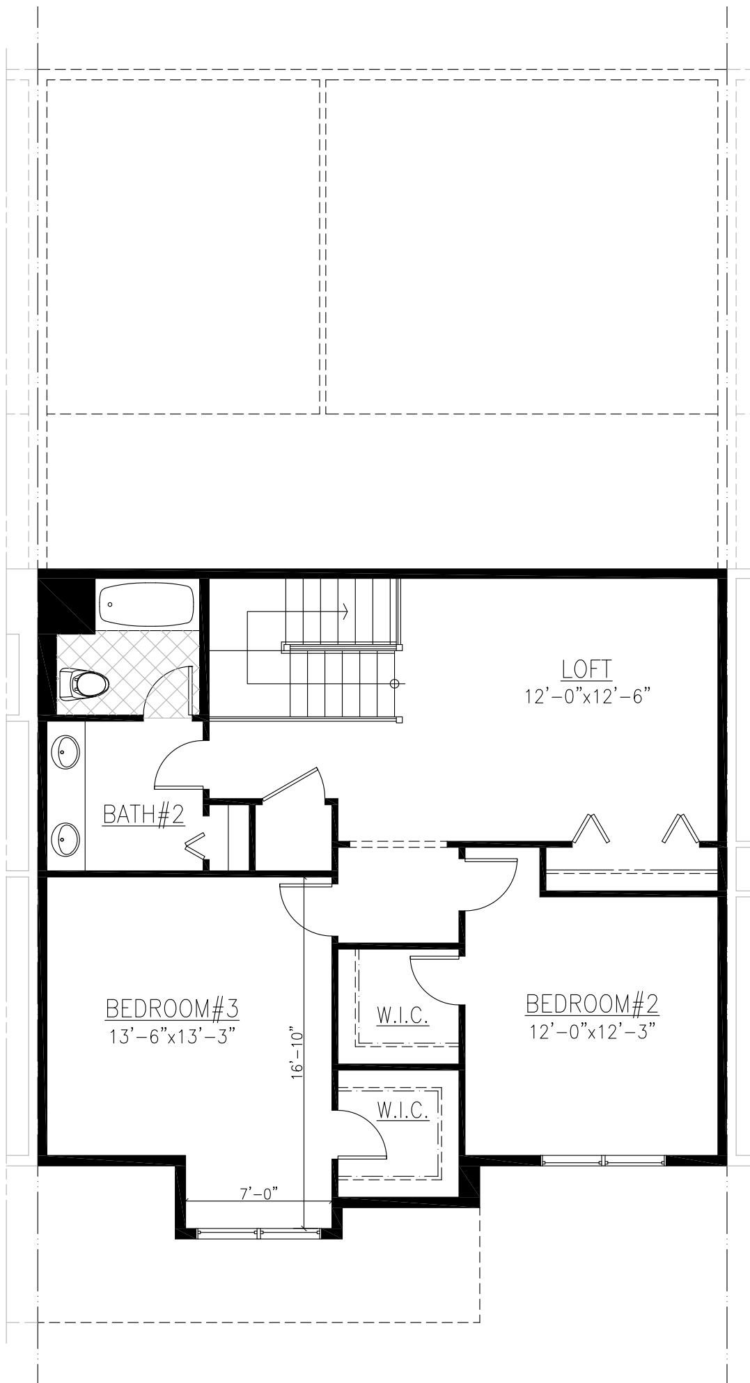
Second Floor Plan Drawing
