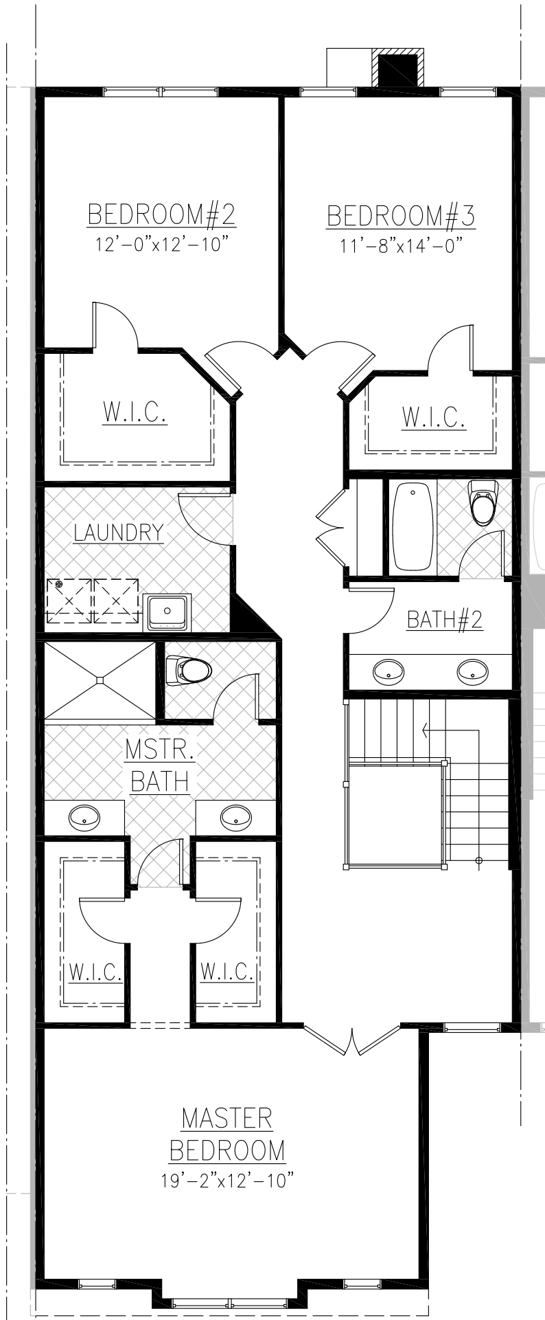
Second Floor Plan Drawing
